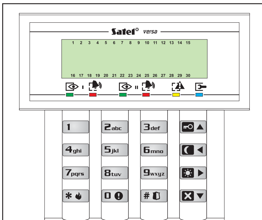
Rys. 1. Manipulator VERSA-LCD.
